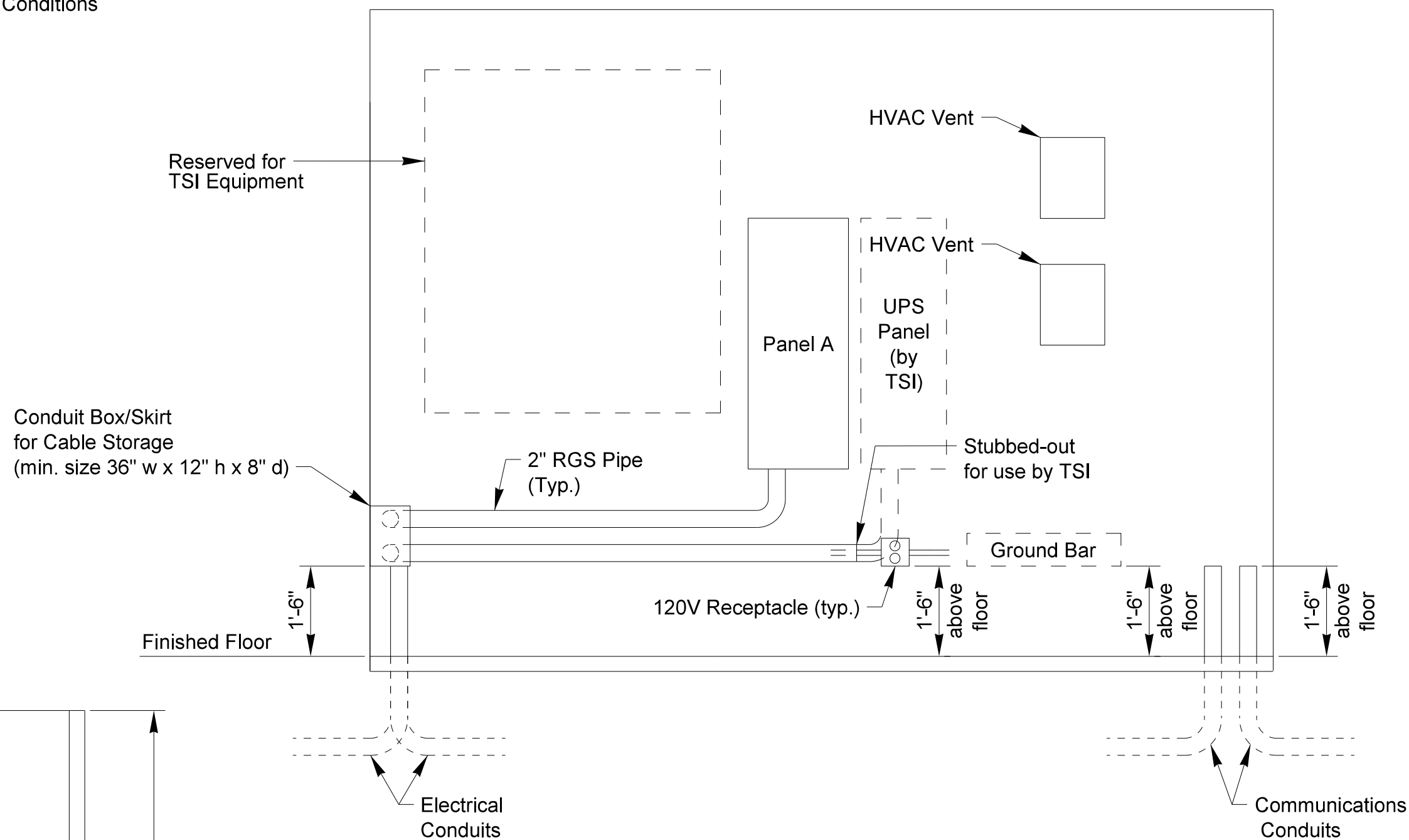
Interior Back Wall Detail
