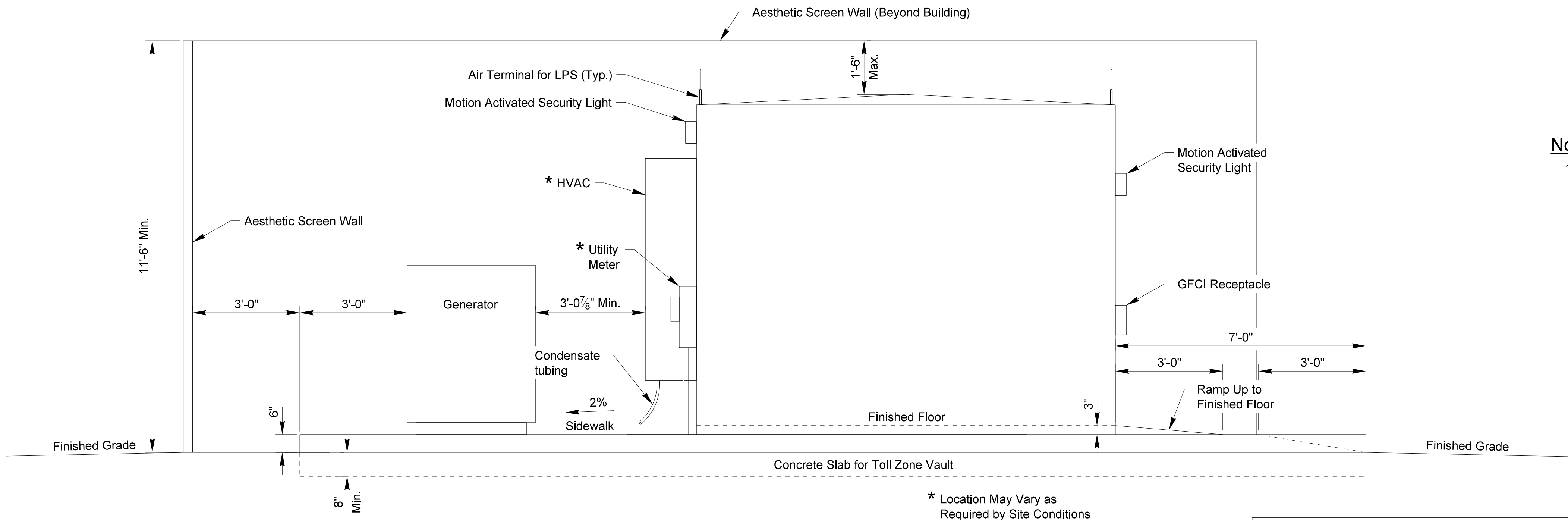
Side Elevation
